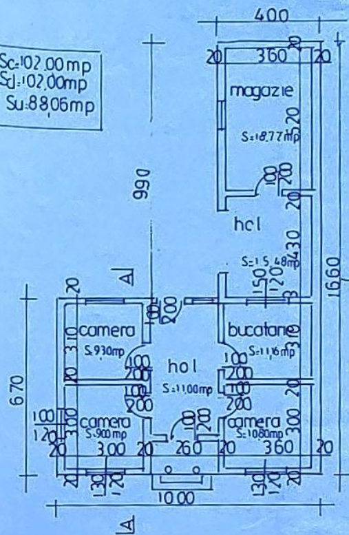
● PLAN PARTER C+ 1:100
