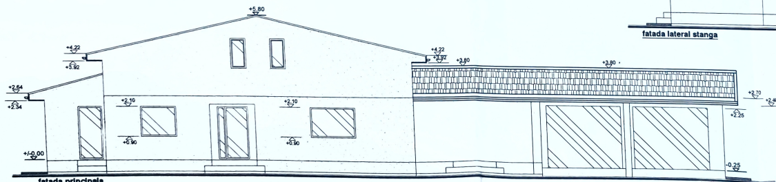
fatada principala
