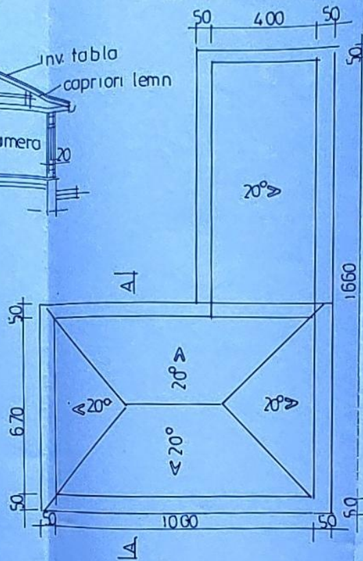
● PLAN ACOPERIS 1:100
